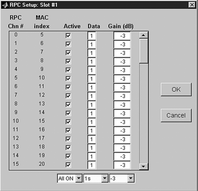
Figure 6. Forward link reverse power control setup table for slot #1
